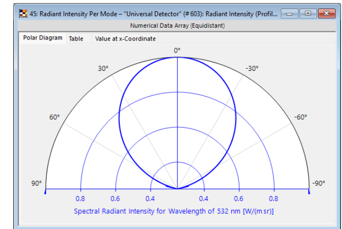
Radiant intensity
